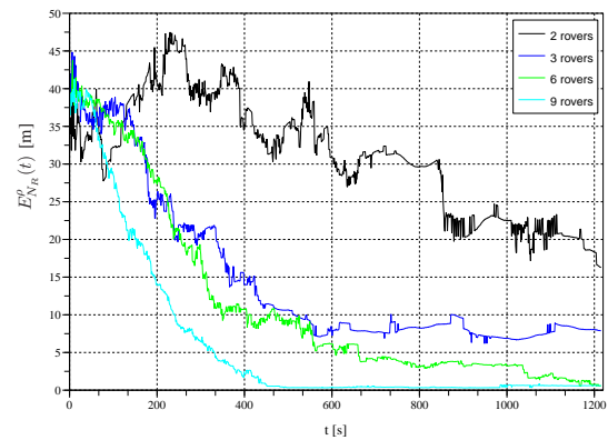
Fig. 5. Experiment 4: average localization errors.
