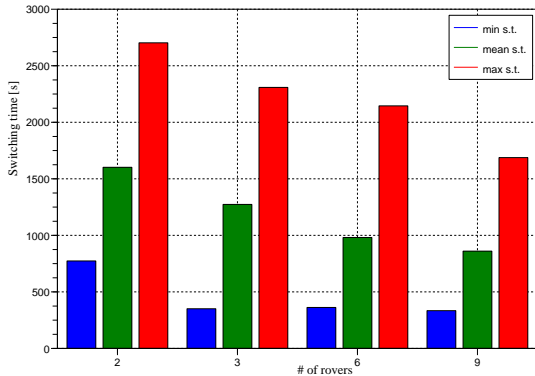
Fig. 6. Experiment 4: switching to position tracking times for groups of rovers of increasing cardinality.
