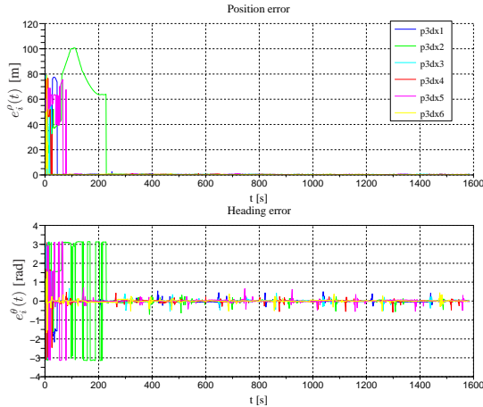
Fig. 1. Experiment 1: localization errors.
