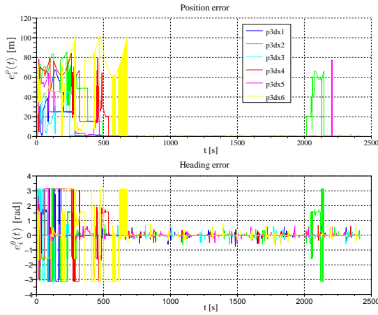
Fig. 3. Experiment 3: localization errors.
